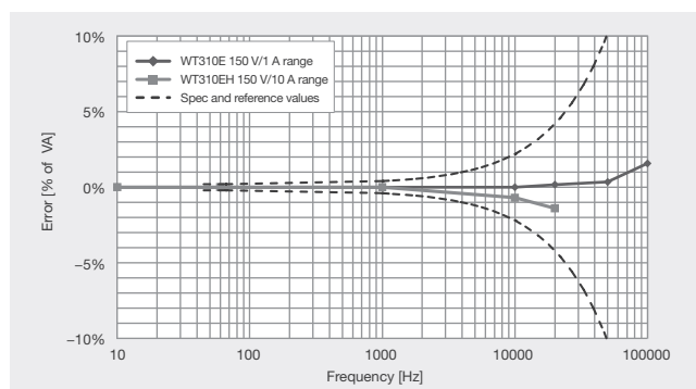
Example of frequency versus power accuracy characteristic (power specification for \cos\theta = 0 )
